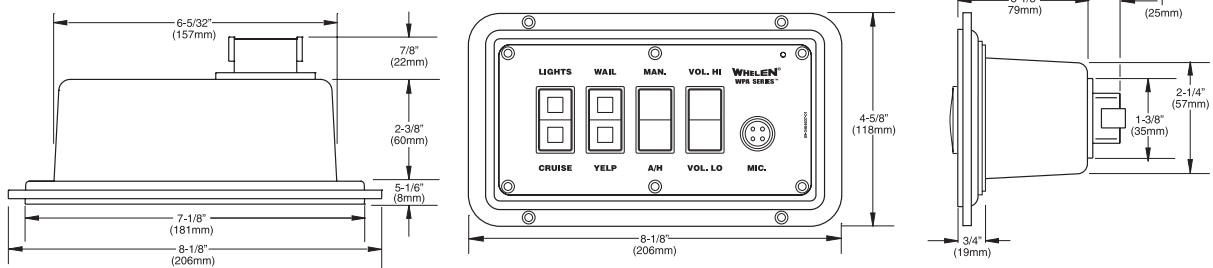
WPA3FM with Flush Mount
