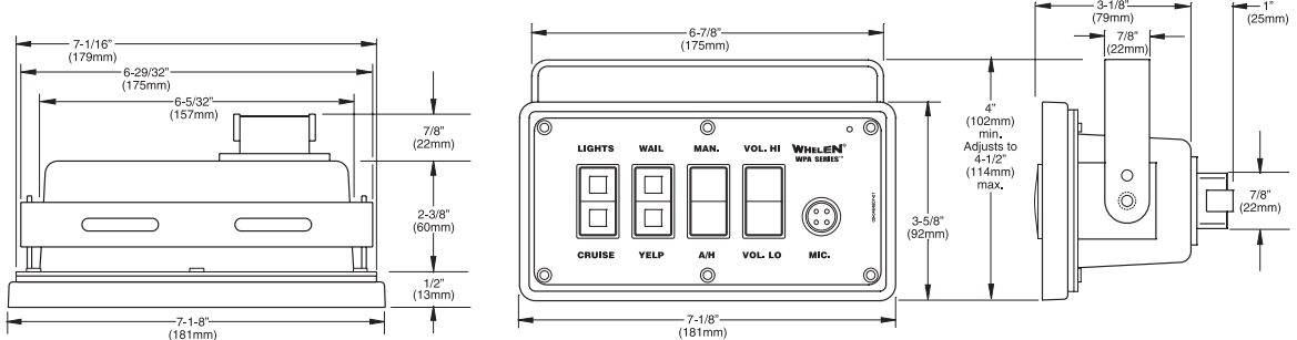
WPA3BM with Bail Mount
